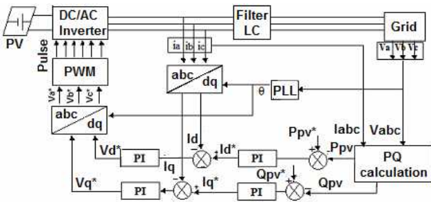
Fig. 4. PV system model
