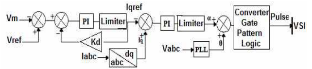
Fig. 6. Control bloc of STATCOM
