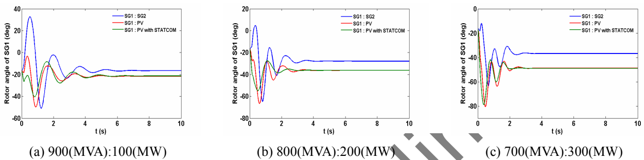
Fig. 14. Rotor angle of SG1 for different power source: SG1 (MVA) : PV (MW) or SG2 (MVA)
