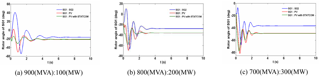
Fig. 10. Rotor angle of SG1 for different power source: SG1 (MVA) : PV (MW) or SG2 (MVA)
