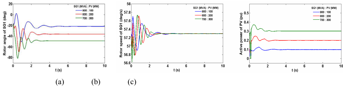
Fig. 7. (a) Rotor angle of SG1 for various PV capacity; (b) Rotor speed of SG1 for various PV capacity; (c) Active power of PV for various PV capacity
