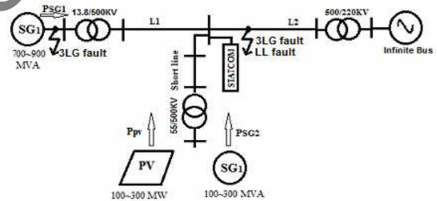
Fig. 3. Power system model
