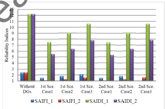
Fig. 3. Reliability indices under different scenarios
