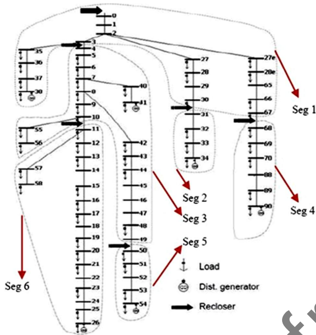
Fig. 2. Network segments defined by dashed lines
