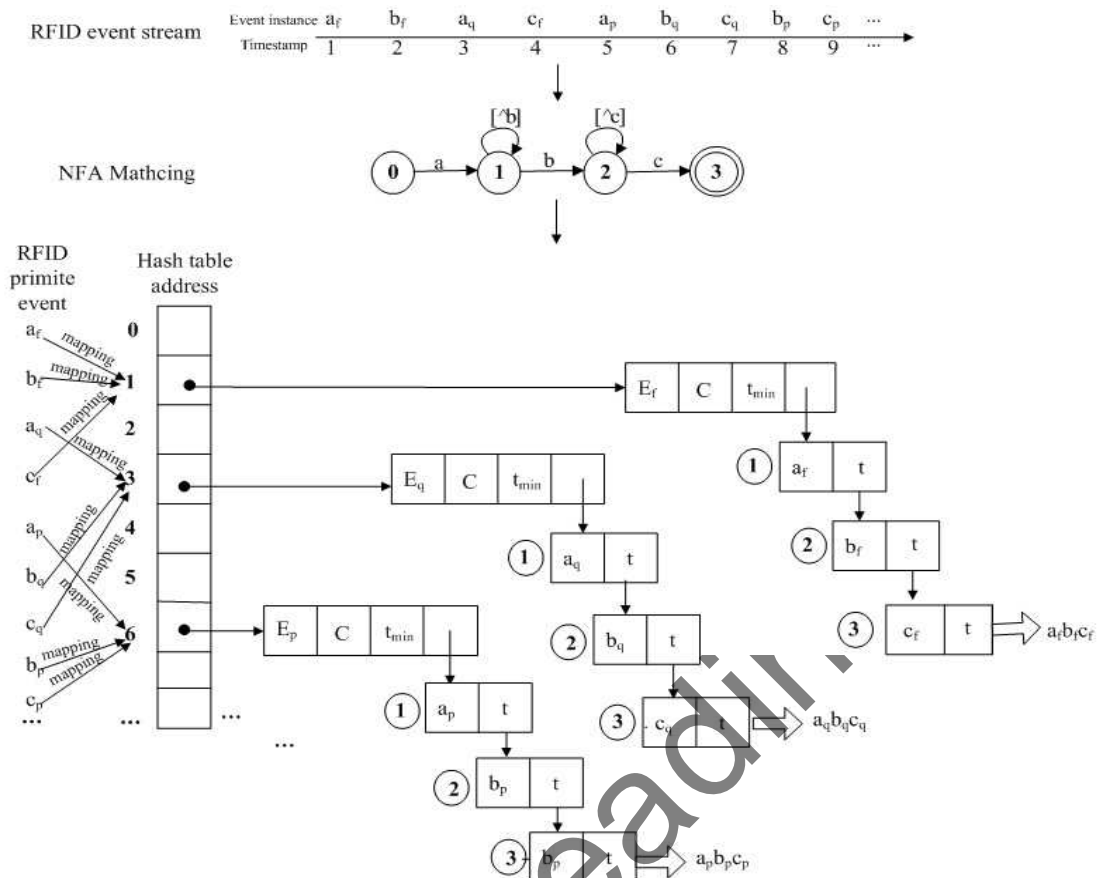
Fig. 2. Detection process of NFA-HTS algorithm
