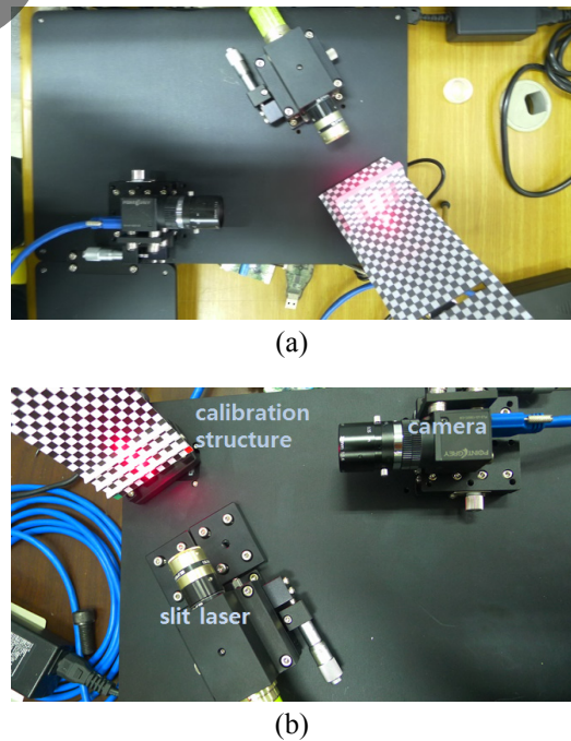
Fig. 3. Experimental setup of structured light stripe system configuration with a camera, a slit laser and a calibration structure: (a) calibration structure with multiple slits; (b) calibration structure with multiple vertical planes
